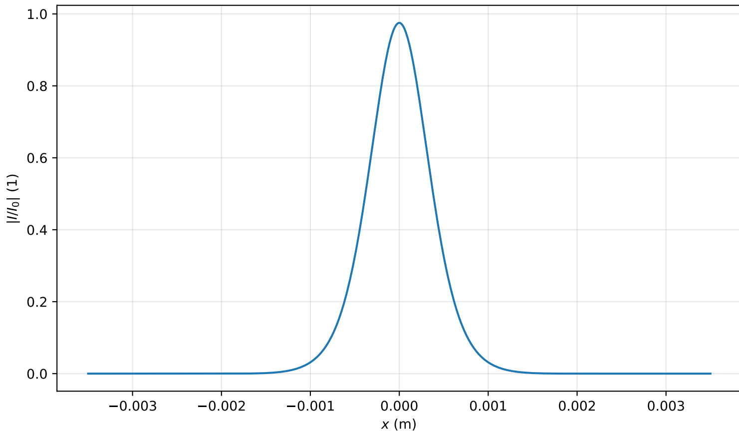
Intensity profile I(x, y = 0, z = 1.433m)/I_0 , P_{in}=0.5P_{cr} , artificial time
